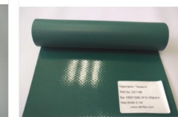
DG-K001: wader material, thickness 0.65mm
